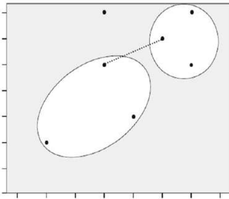
Figure 38: Single – Linkage type of agglomerative HCA
